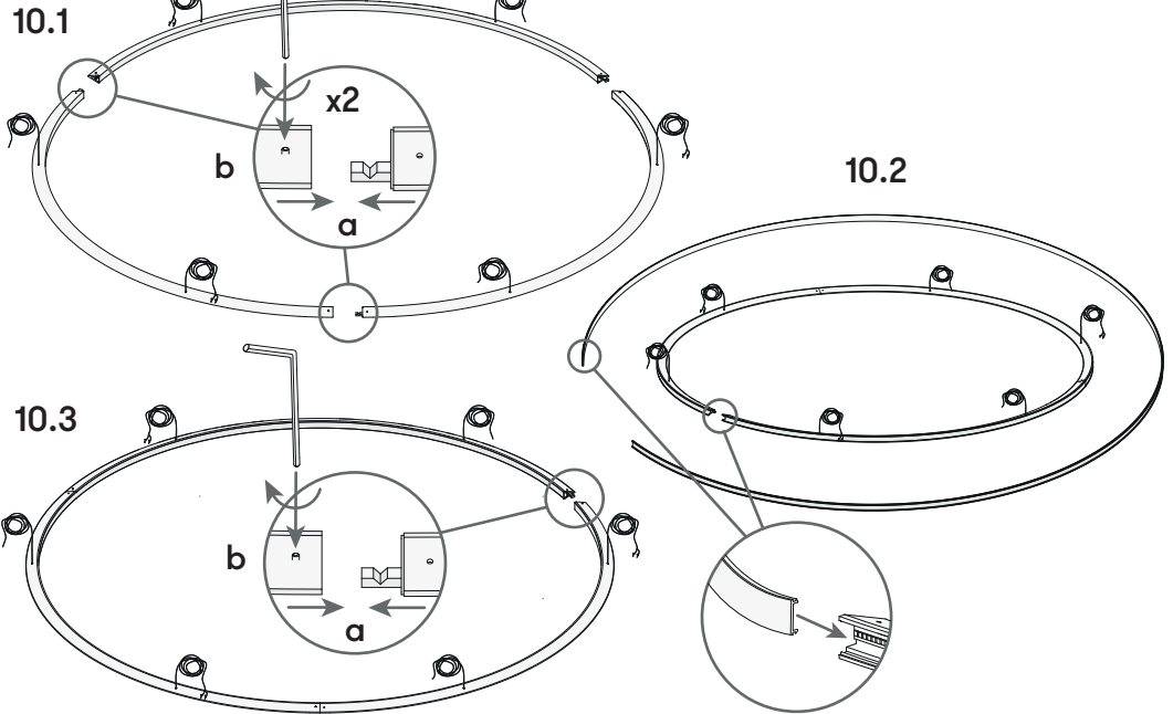
Outward Ø2000
